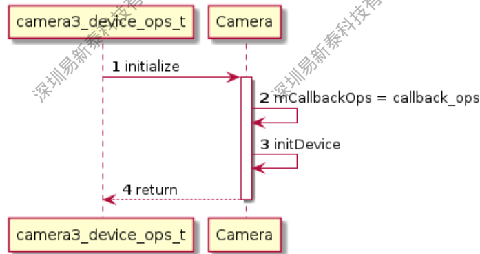
图 5-5: camera3_device_ops_t-initialize 流程图
